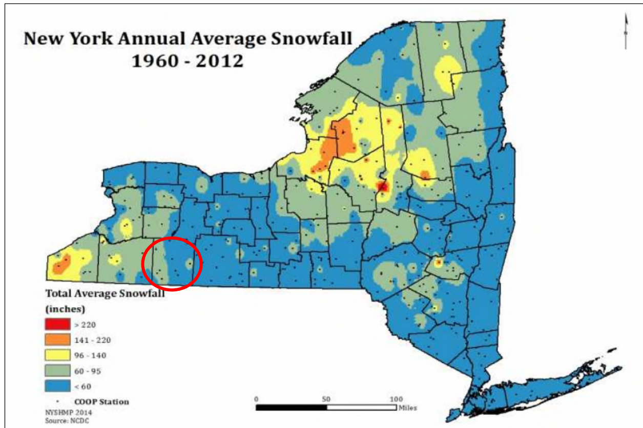
Figure 5.4.10-1. Annual Average Snowfall for New York State
